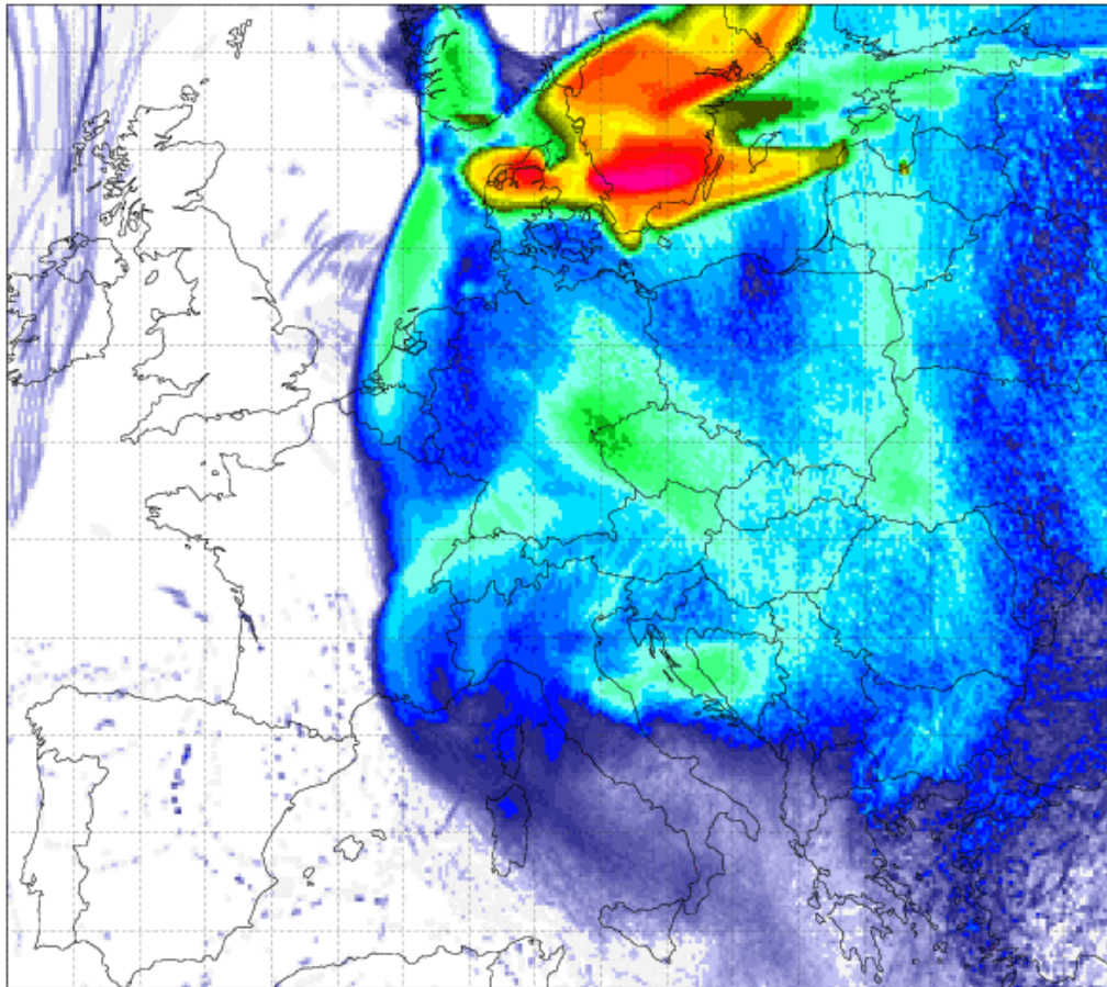
Fennovoima-1 Deposition from a 173.70 PBq release of Cs-137 Simulation start 19950507 21 Actual time 19950522 21
